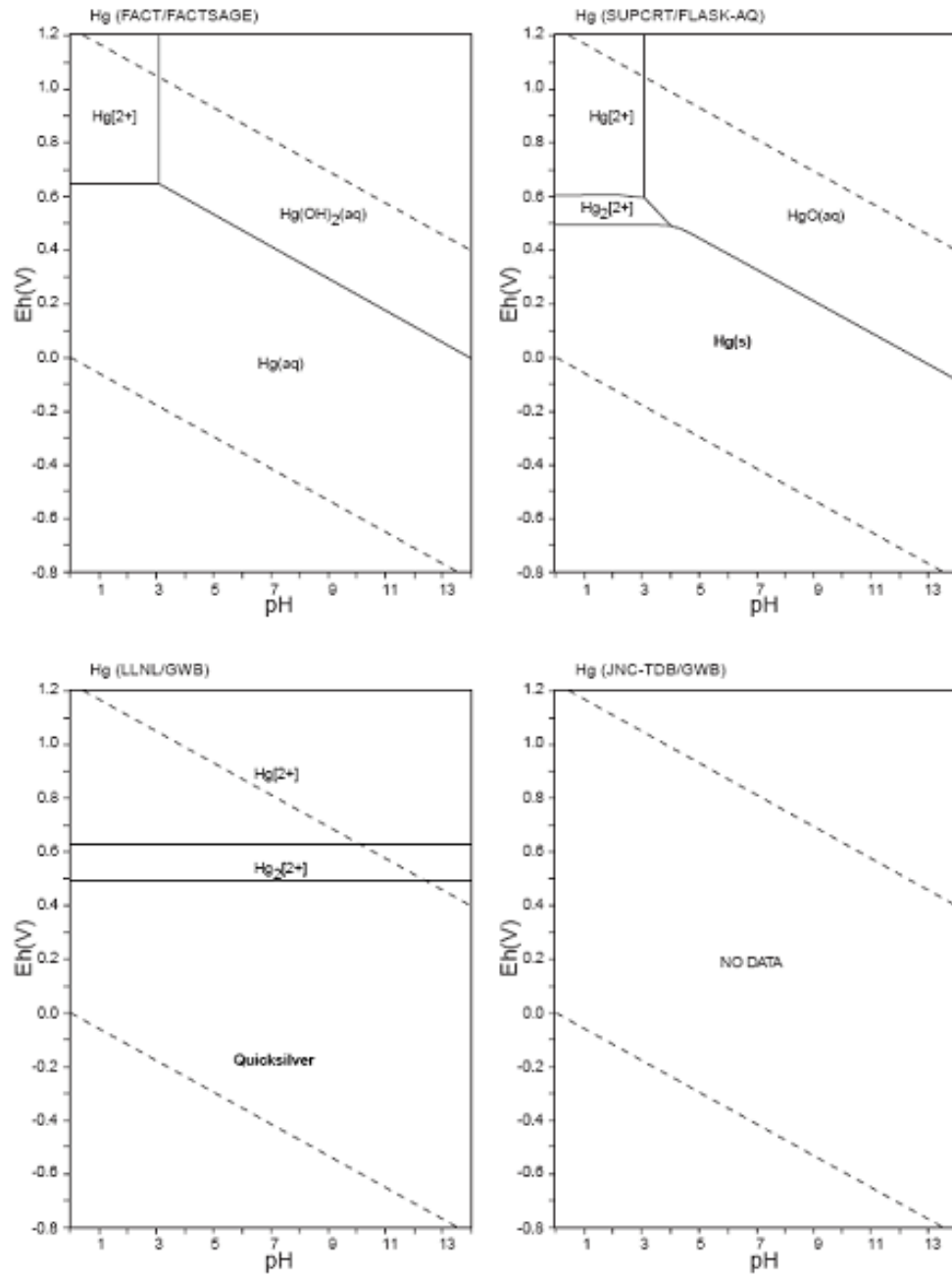
Figura 18. Diagramas Eh-pH del sistema Hg-O-H (1) \Sigma\text{Hg} = 10^{-10} , 298.15K, 105 Pa
