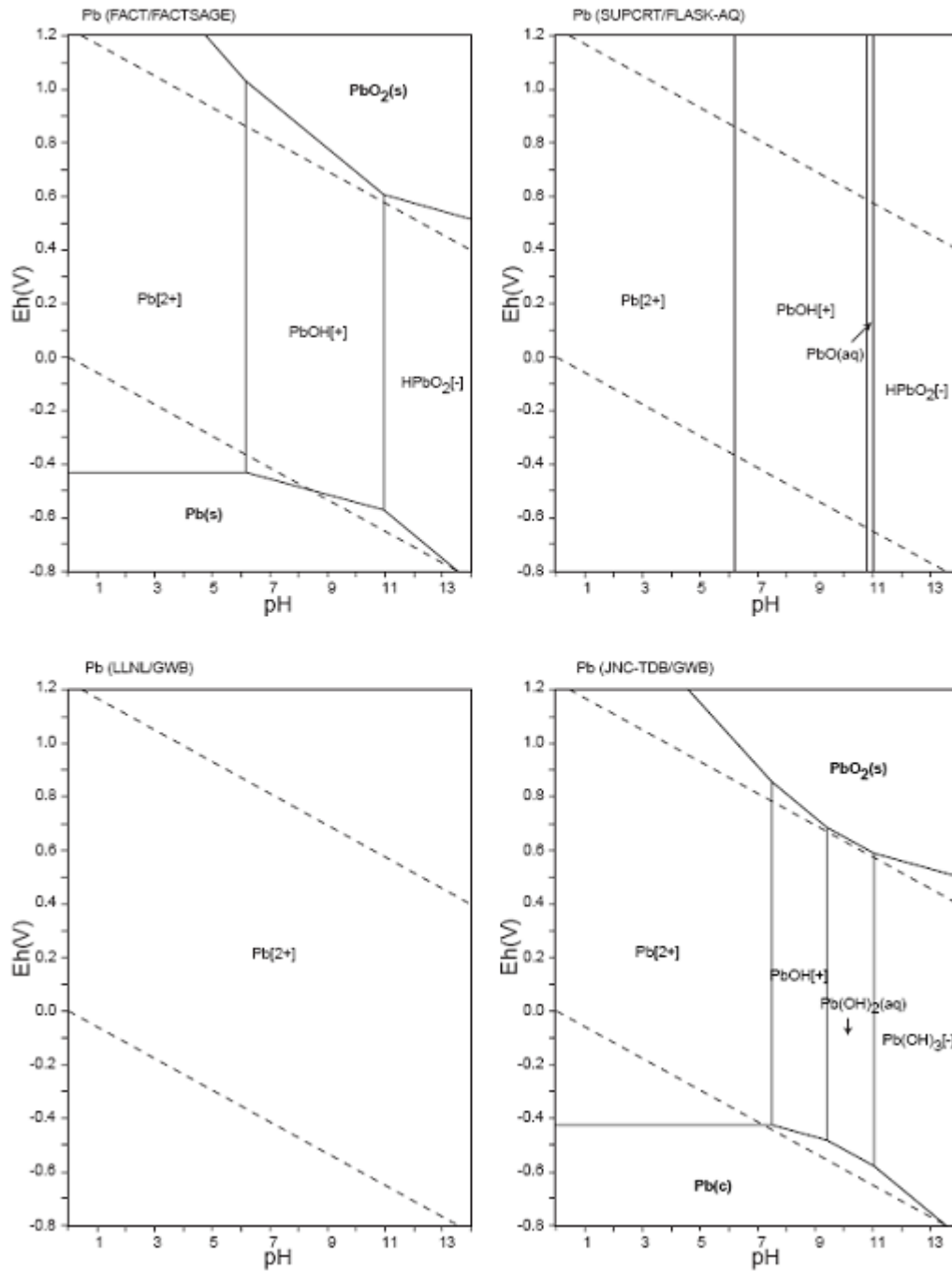
Figura 16. Diagramas Eh-pH del sistema Pb-O-H (1) \Sigma Pb = 10^{-10} , 298.15K, 105 Pa
