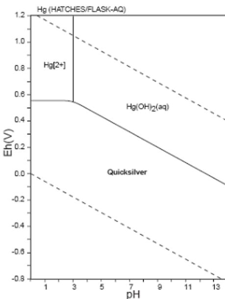
Figura 19. Diagramas Eh-pH del sistema Hg-O-H (2) \Sigma\text{Hg} = 10^{-10} , 298.15K, 105 Pa
